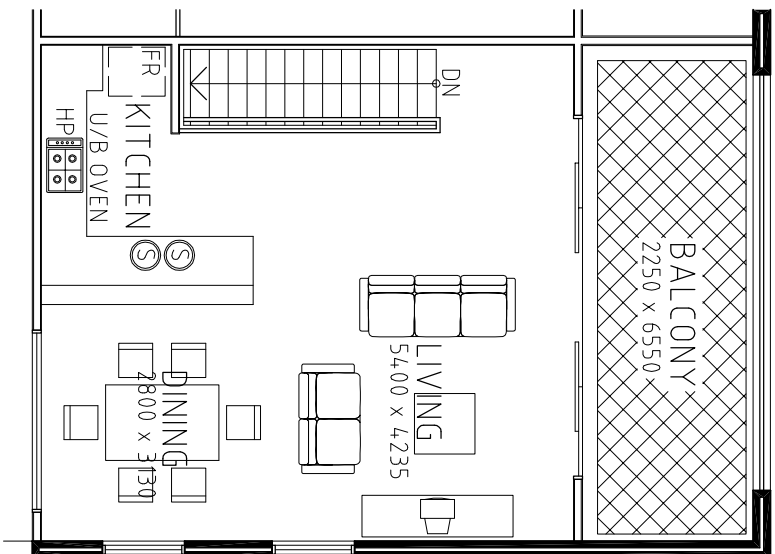
SECOND FLOOR SCALE 1:100
